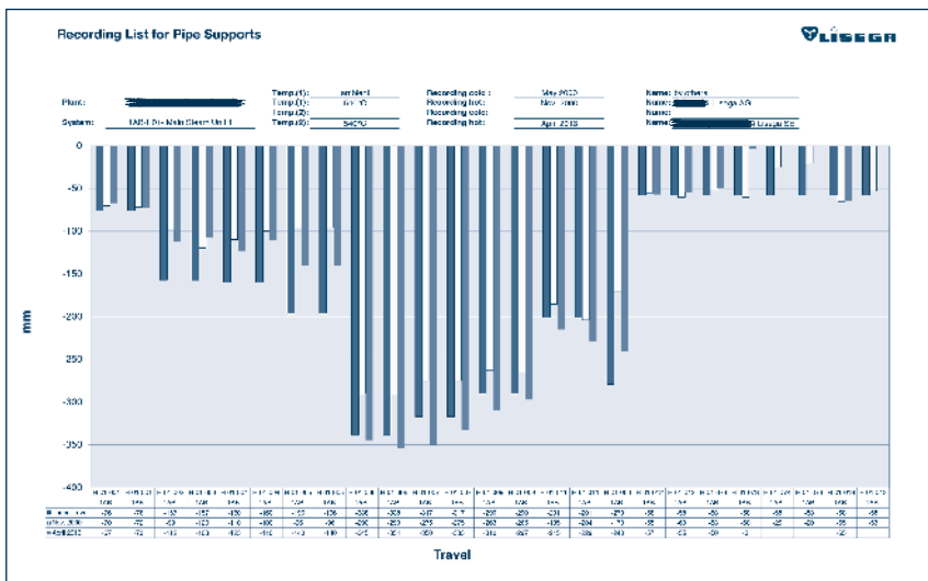
Cold/hot position of a pipe system
