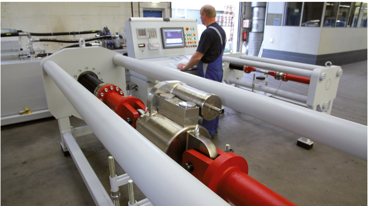
Test bench for snubbers
