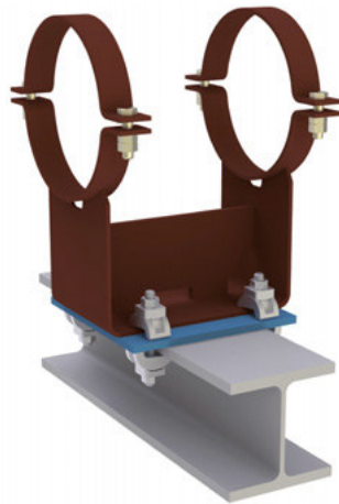
Example of use: Attachment of clamp base to steel beam
