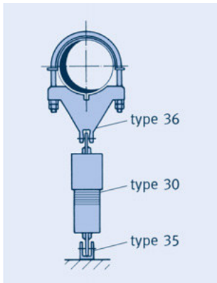
Typical installation situation for type 30
