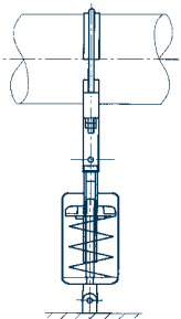
Angulating spring support type 20
