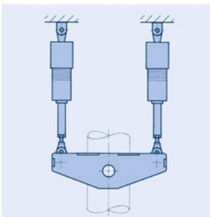
Type 34 with snubbers type 30 and twist restraints
