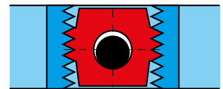
b) Guide pin lies at bottom: Set load of constant hanger is smaller than weight applied. Loosen connecting rod or increase set load.
