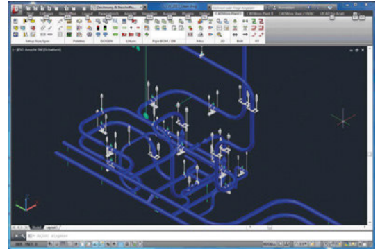
LISEGA supports in CADWorx®
