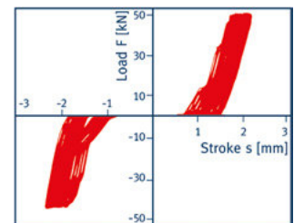
Measured force/travel path with oscillating loads > nominal load
