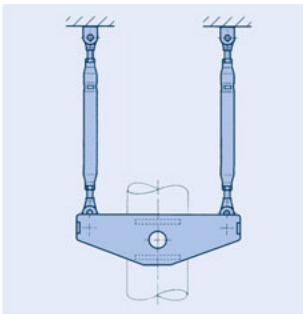
Type 34 as axial stop with spacer
