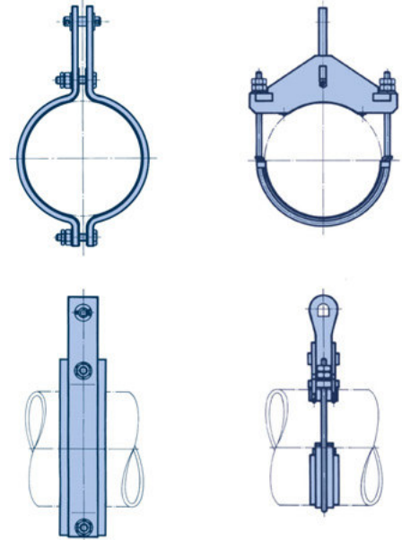
Type 43 with inlay plate
