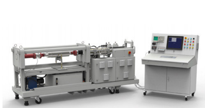
Mobile LISEGA 50kN snubber test bench PR50
