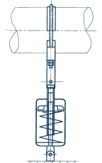
Angulating spring support type 20
