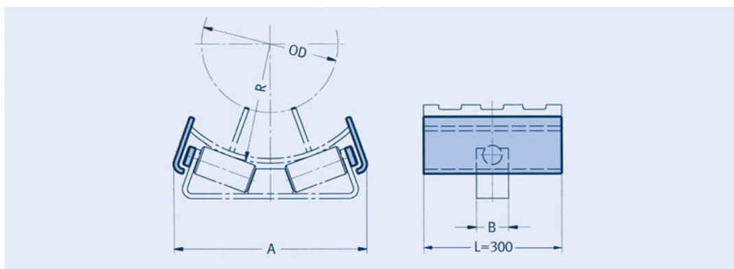
Lift-off restraints type 55 08 19 to 55 12 19
