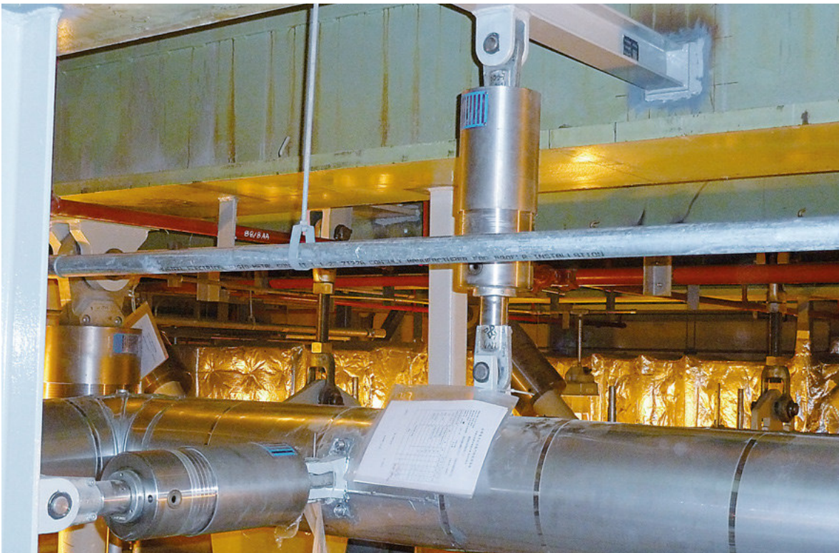
Pipe system secured with snubber type 30 on dynamic clamps type 36
