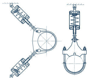
Sway brace type 27 angled arrangement
