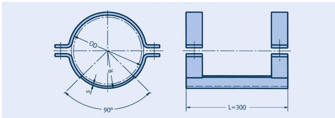
Pipe trays with clamps type 54 06 39 to 54 81 39
