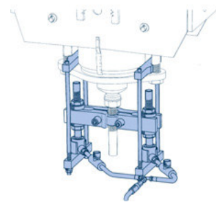
Installation device, used to relieve the adjusting nut
