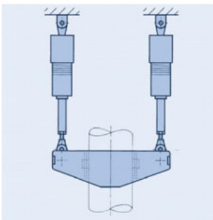
Type 34 with rotated trunnion hole and snubber type 30
