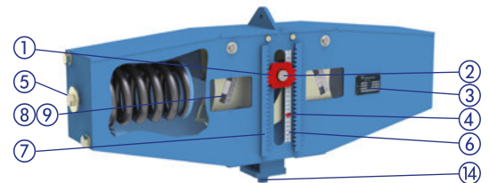
Low profile constant hanger type 18
