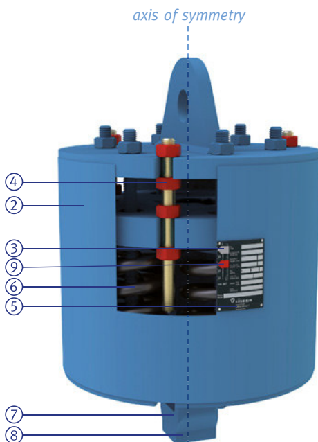
Spring hanger type 22
