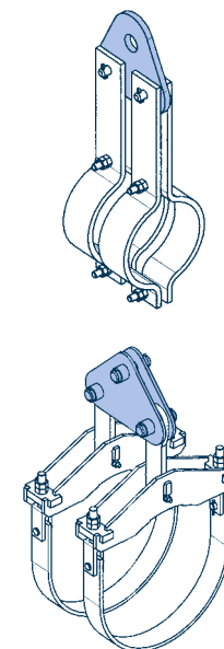
Connection plates type 77 on pipe clamps type 43/44
