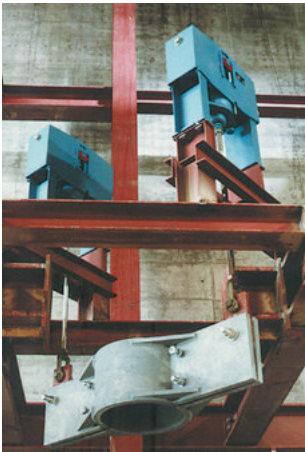
Support for a vertical pipe section with special design type 45
