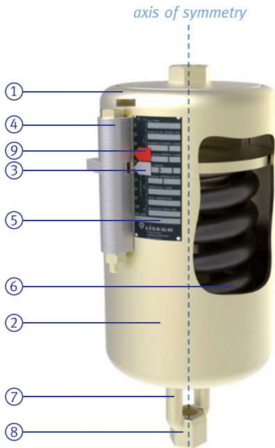
Spring hanger type 21
