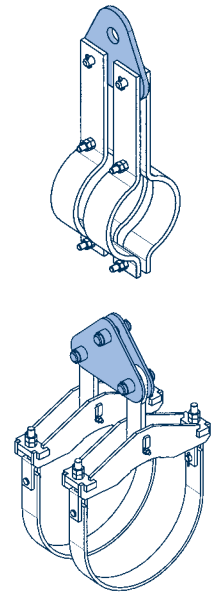
Connection plates type 77 on pipe clamps type 43/44
