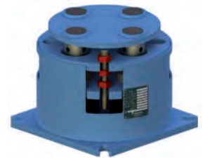
Type 28 with embedded slide plates
