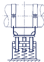
Spring support type 28
