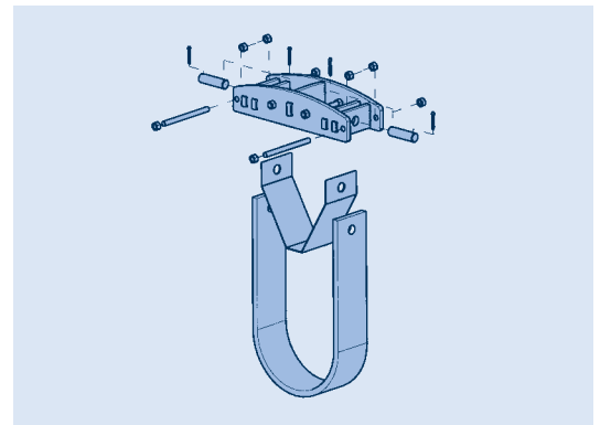
Installation of type 44 for temperatures over 1110°F [600°C]
