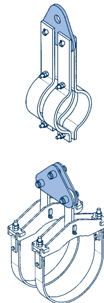
By coupling two pipe clamps with connection plates type 77 the loads can be doubled. A selection can be found on page 4.67.
