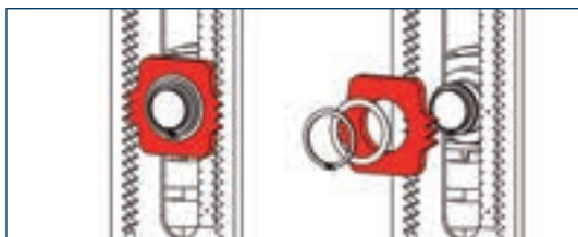
Blocked condition ① Dismantling of the outer locking ring and blocking device
