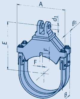
type 37 ...8/9
