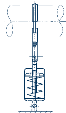
Angulating spring support type 20
