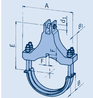
type 36 ... 4/5
