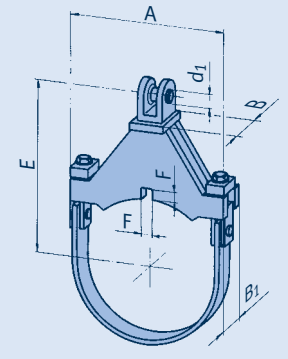
type 37 .. .1/2/3/4/5/6
