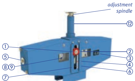
Constant support type 19
