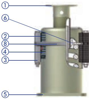
Spring support type 29 (blocked)
