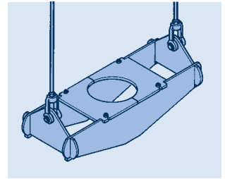
Riser clamp type 46 with connection components
