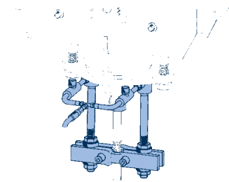
Installation device, used to relieve the load adjustment bolts
