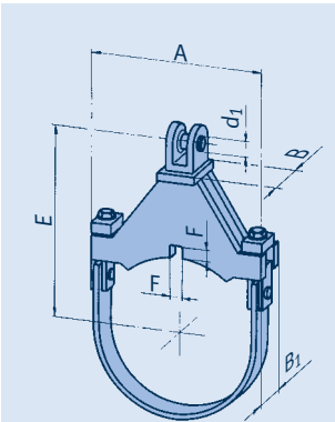
type 37 .. .1/2/3/4/5/6
