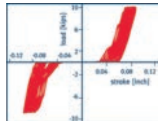
Measured force/travel path with oscillating loads > nominal load
