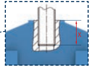
Min. thread engagement depth „X“ of upper connection (see selection table type 11, page 1.15)
