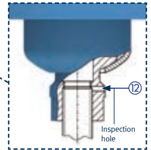
Min. thread engagement depth of connection rod in load tube
