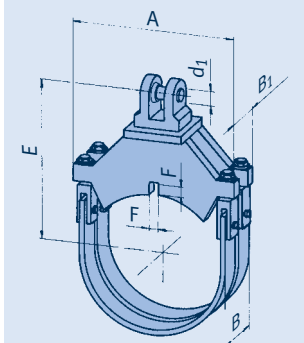
type 37 ... 7/8
