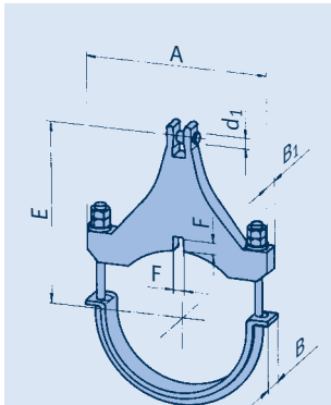
type 36 ... 1/2/3
