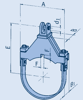
type 37 ... 1/2/3/4/5/6
