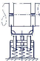
Spring support type 28
