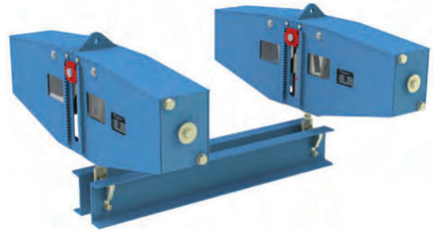
Constant hanger trapezes type 79 D3 17 to 79 93 17
