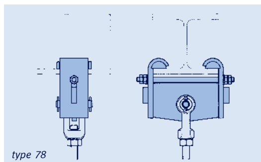
Standardized connection possibilities
