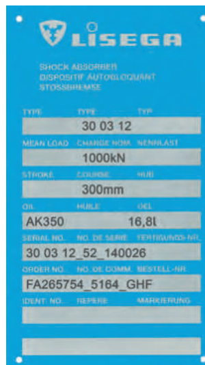
Name plate type 30
