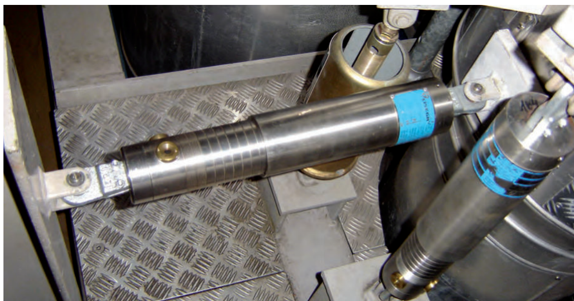
Use of snubbers type 30
