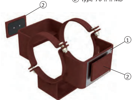
slide bearing / guide through clamp base type 49 .. G3-SP with slide plates
