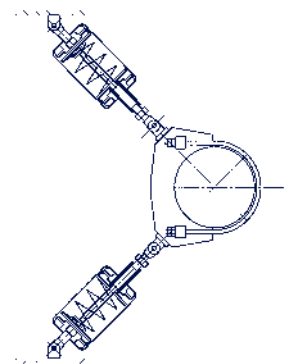
Sway brace type 27 angled arrangement
