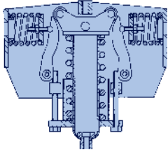
LISEGA constant hanger type 11 standard design
