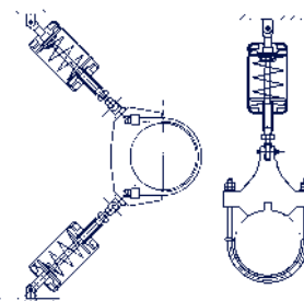
Sway brace type 27 angled arrangement
