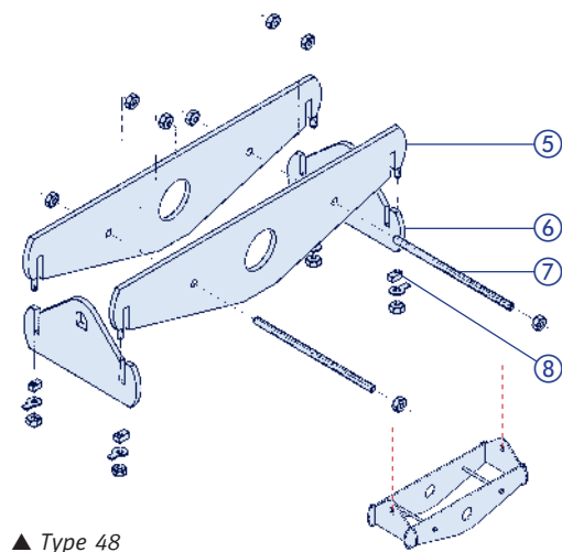
Riser clamp type 48 with connection components
