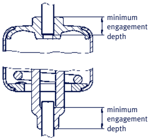
Minimum engagement depth of threaded rods by example of type 21
