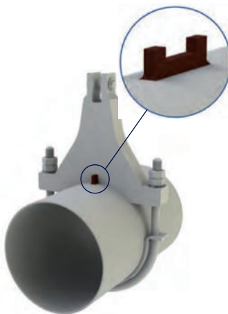
Type 36 with shear lug type 3L
