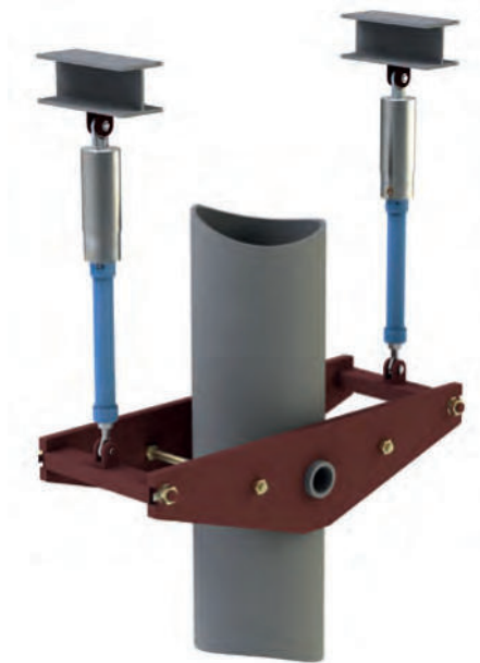
Restraint of a vertical pipe system section by type 30 snubbers with installation extension type 33 and dynamic clamp type 34.
