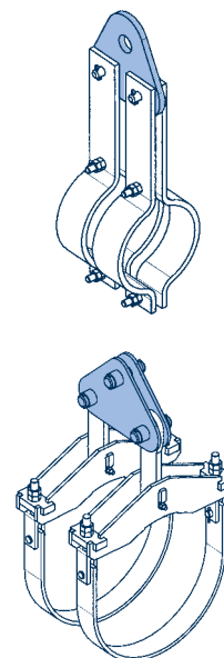
Connection plates type 77 on pipe clamps type 43/44
