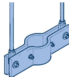
Riser clamp type 45 with connections
