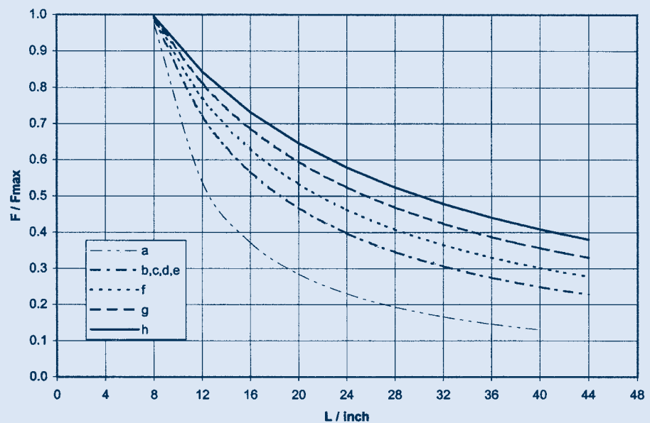
Permissible load in dependence on length of stanchion for slide bearing or fixed point
