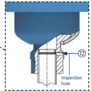
Min. engagement depth of connection rod in load tube
