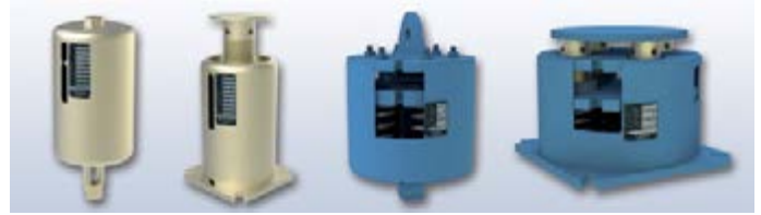
Product Group 2 Spring hangers, spring supports, types 21, 22, 28, 29
