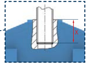
Min. engagement depth „X“ of upper connection (see selection table type 11, p. 1.15)
